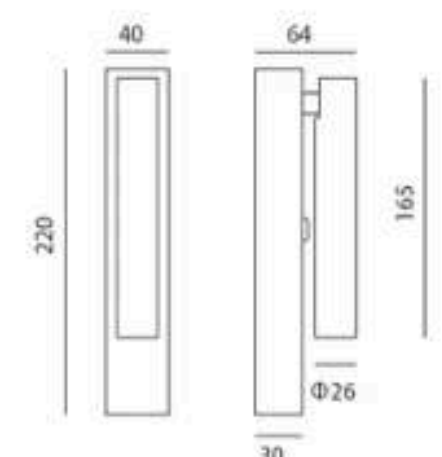
ZT4005-W
