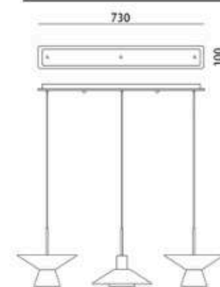
ZT3005-Canopy-L730
