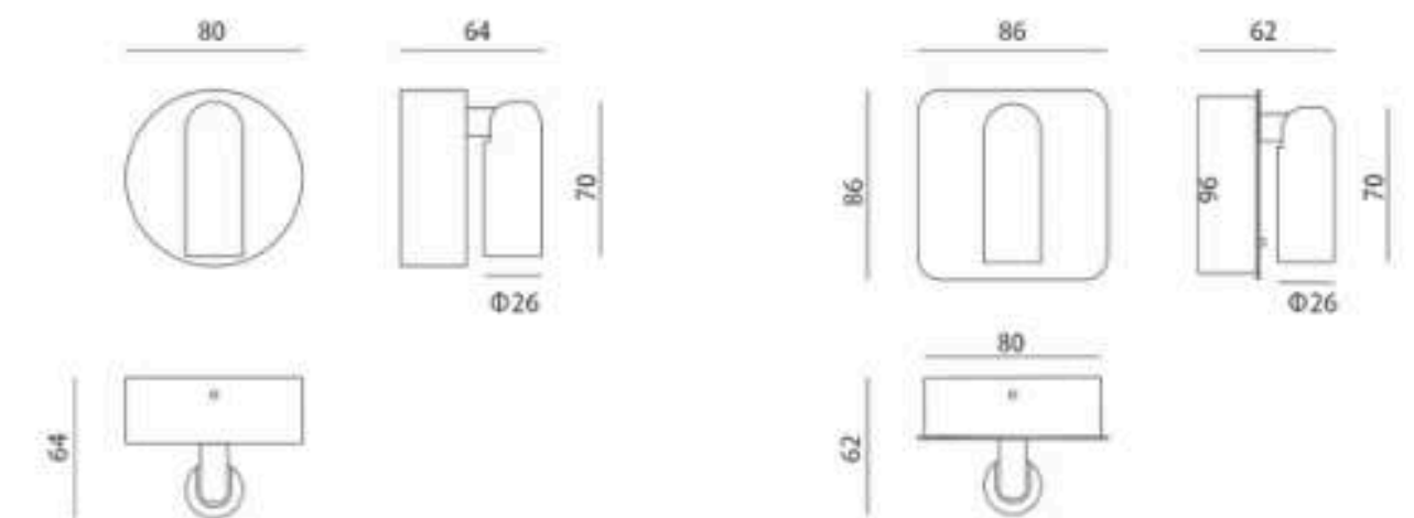
ZT4007-W(A)
