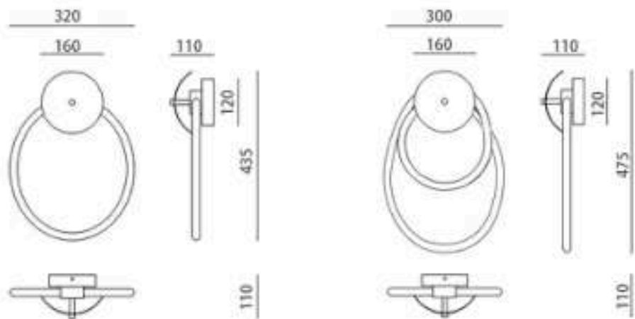
ZT8012-W-S
