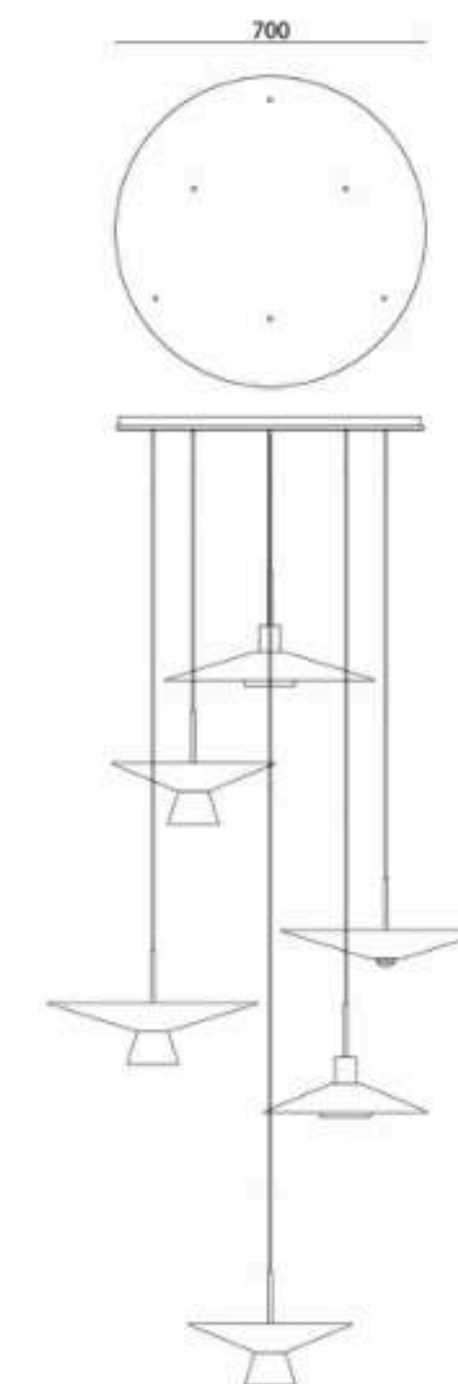
ZT3005-Canopy-D700
