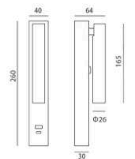
ZT4005-WL
