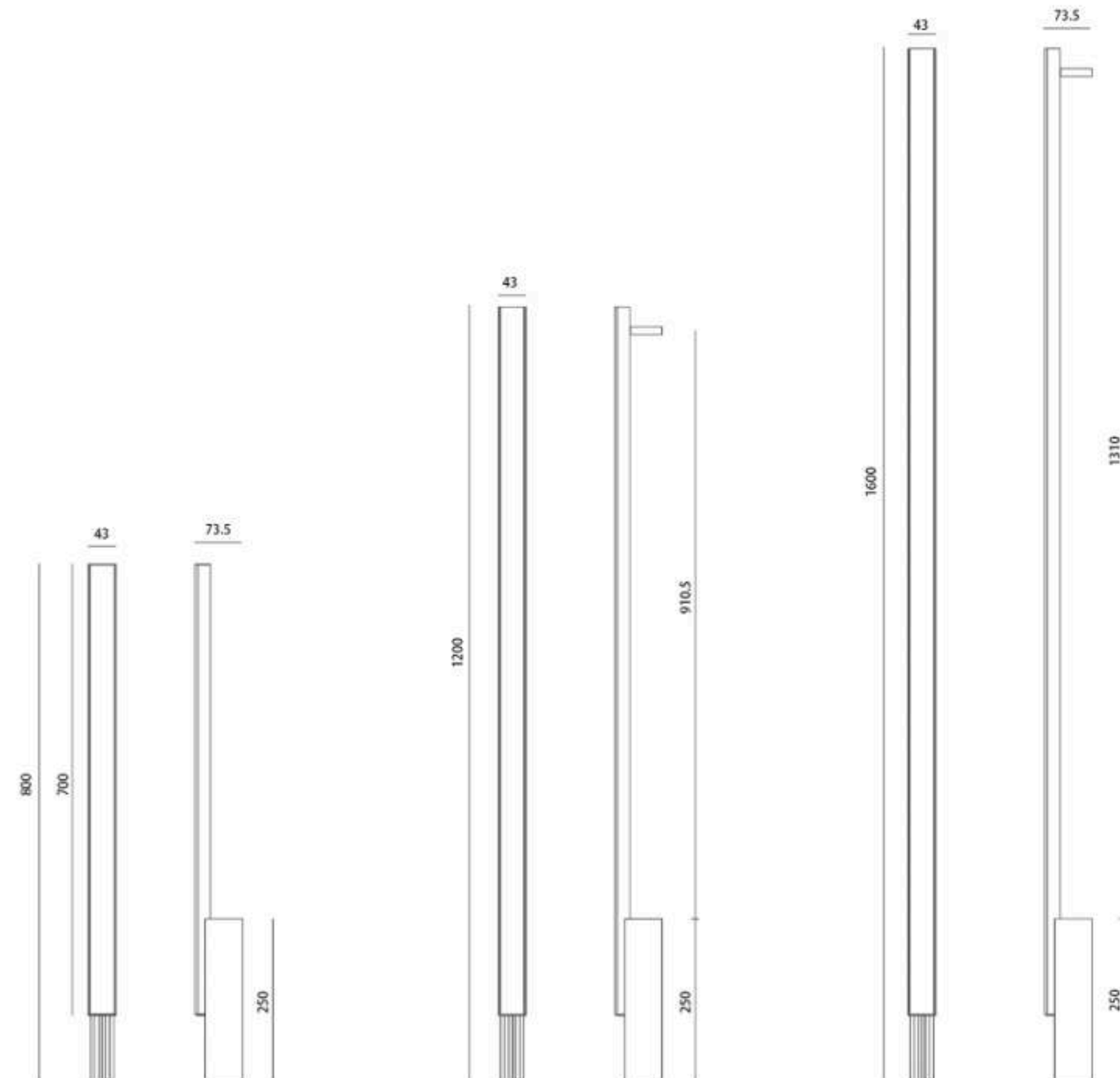
ZT9026-A-800
