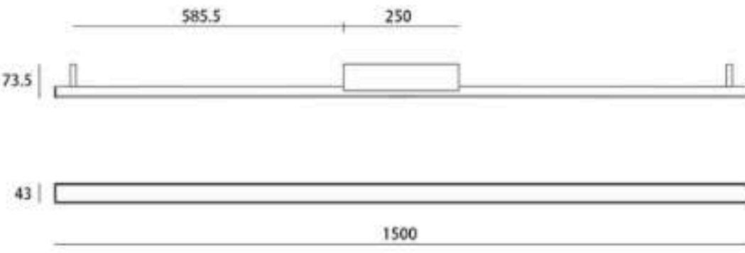
ZT9026-B-1500
