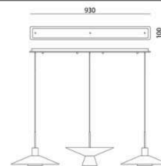
ZT3005-Canopy-L930
