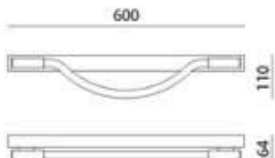
ZT8011-W-S
