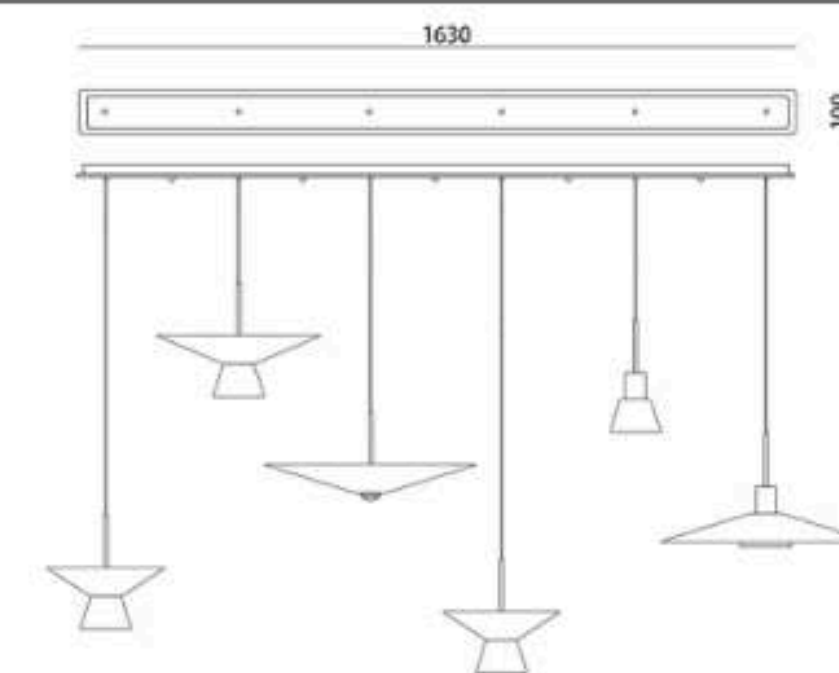
ZT3005-Canopy-L1630
